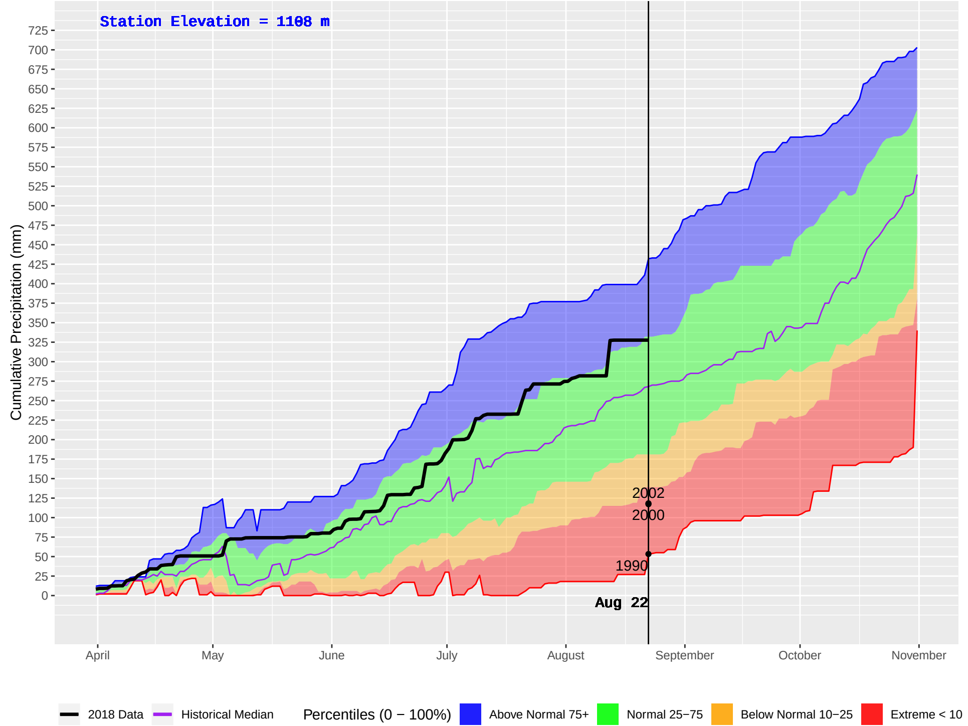
MATHEW (263) : Historical (1987–2016) and Current (2018) Daily Cumulative Precipitation
