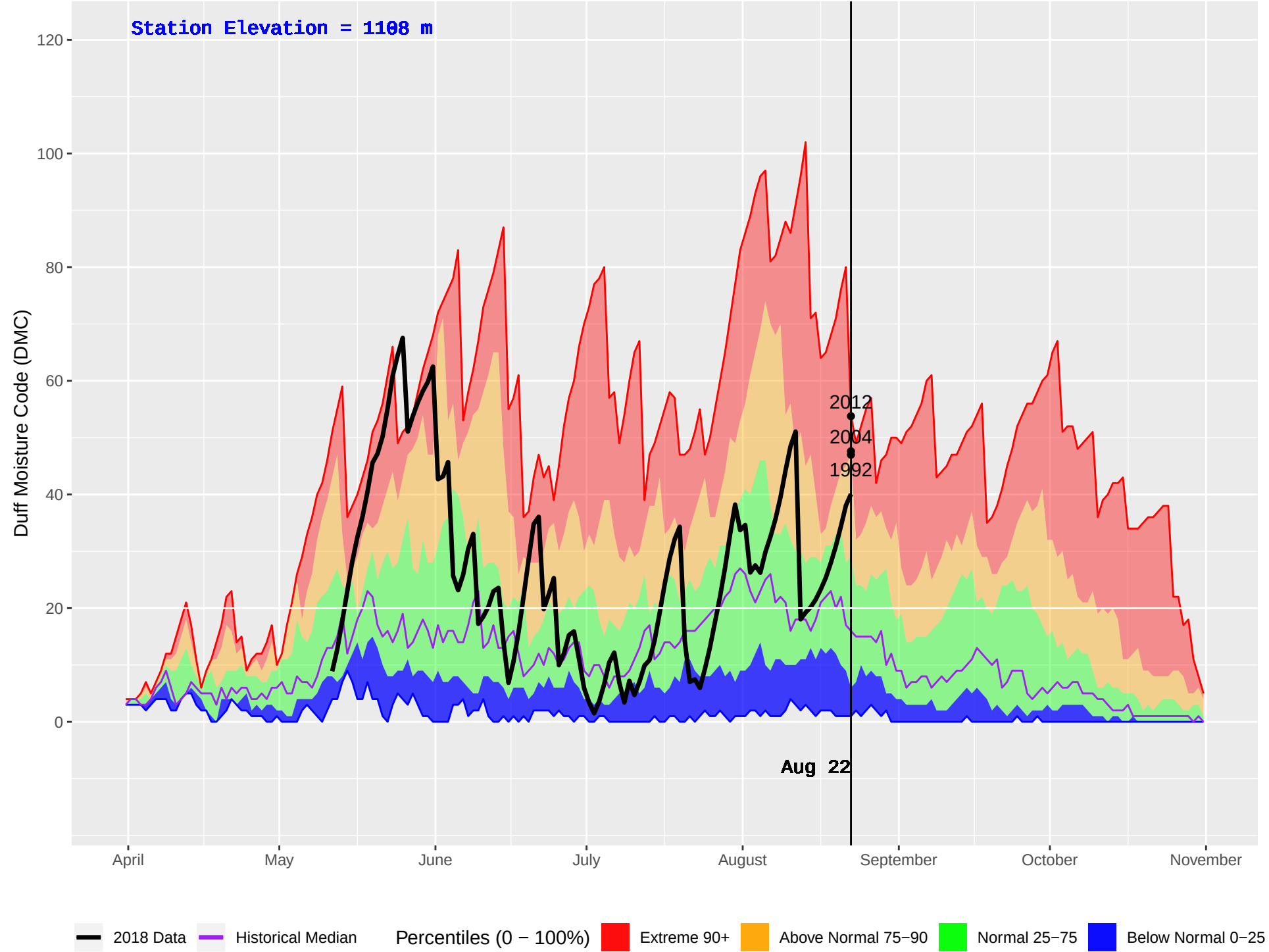
MATHEW (263) : Historical (1987–2016) and Current (2018) Daily Duff Moisture Code (DMC)
