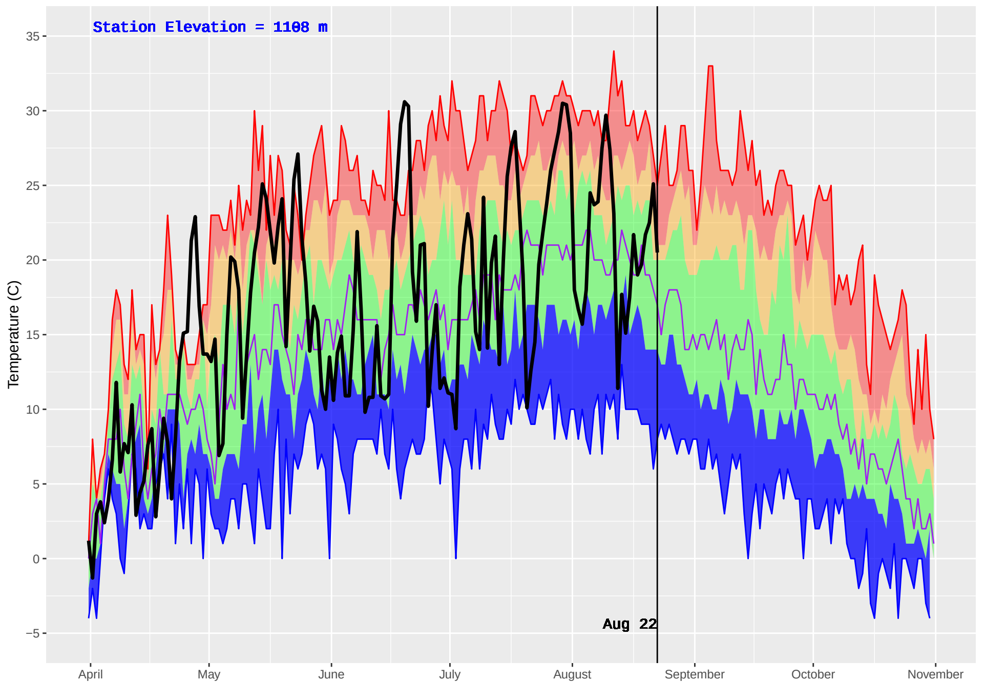
MATHEW (263) : Historical (1987–2016) and Current (2018) Daily Temperature
