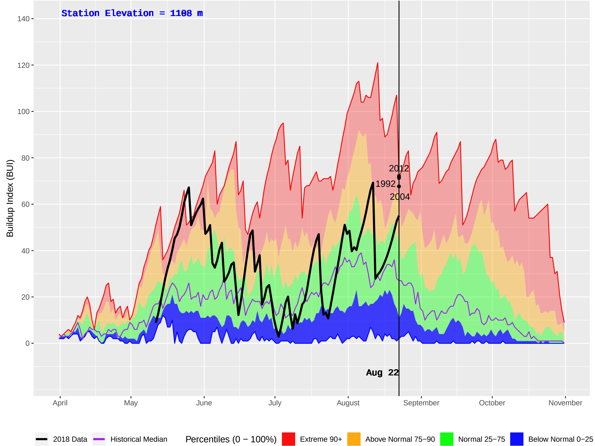
MATHEW (263) : Historical (1987–2016) and Current (2018) Daily Buildup Index (BUI)
