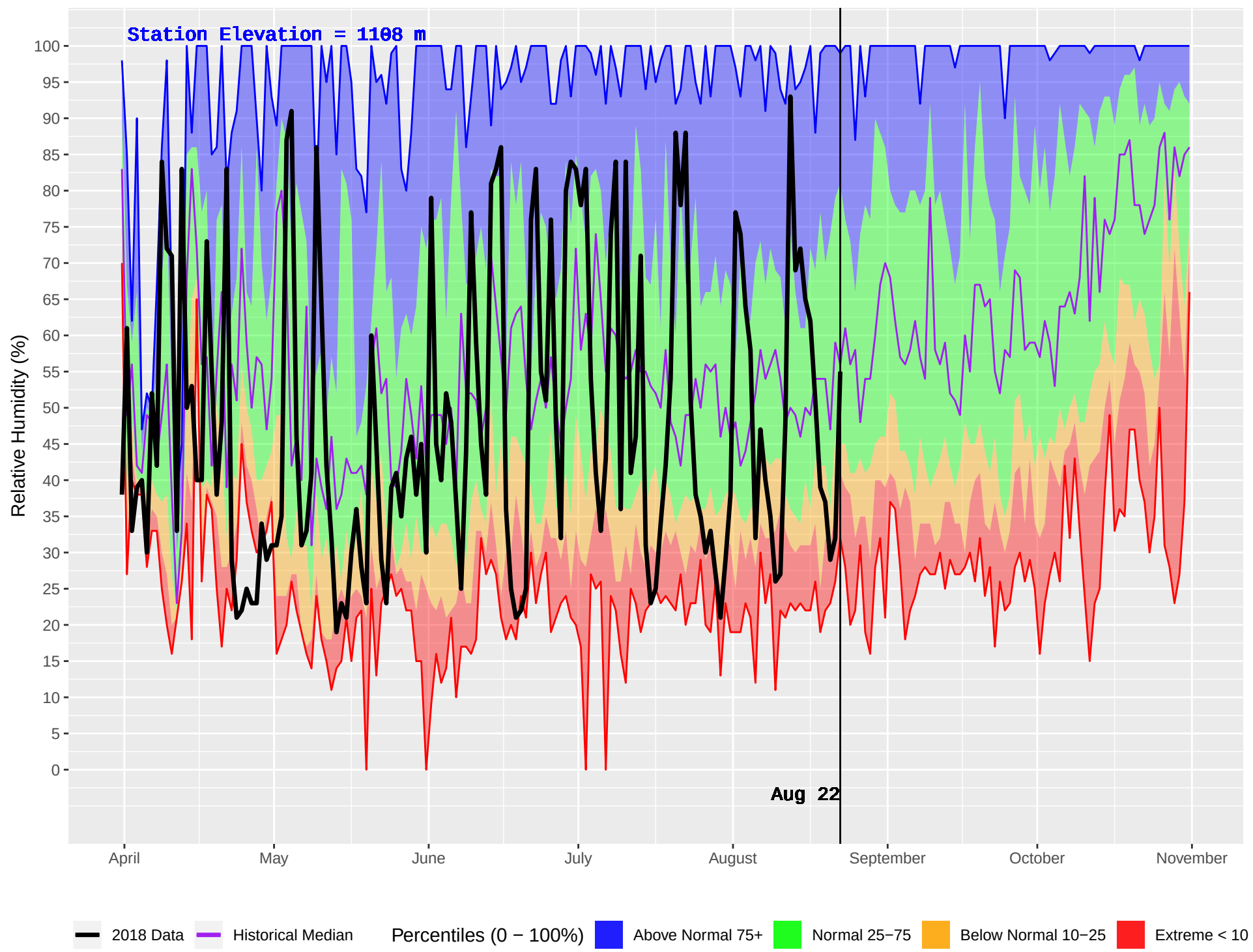
MATHEW (263) : Historical (1987–2016) and Current (2018) Daily Relative Humidity
