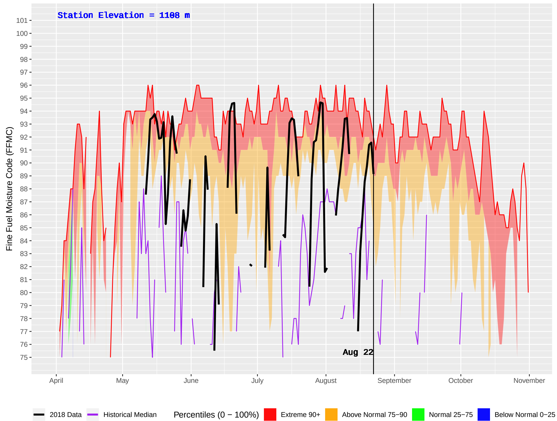
MATHEW (263) : Historical (1987–2016) and Current (2018) Daily Fine Fuel Moisture Code (FFMC)
